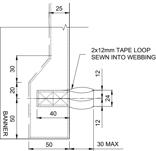
DETAIL 2
