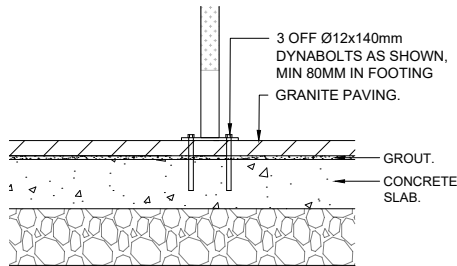
BIKE CHICANE ON GRANITE PAVING
