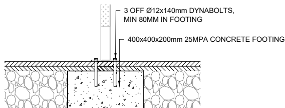
BIKE CHICANE ON ASPHALT
