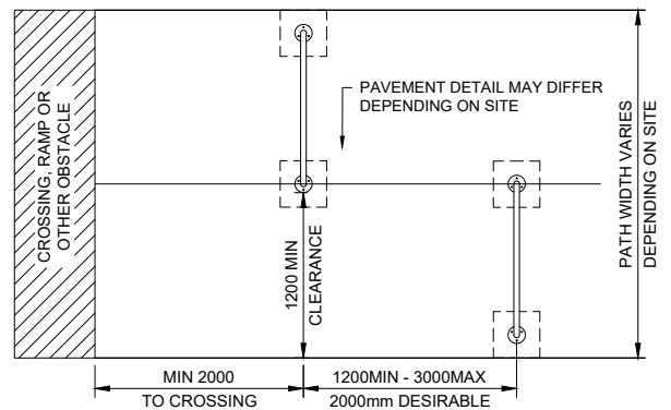
TYPICAL CHICANE LAYOUT
