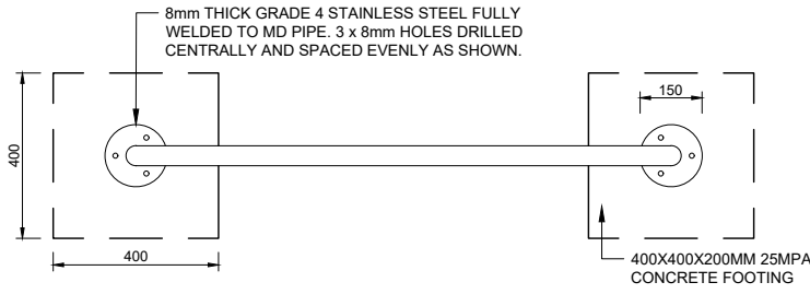
A PLAN
