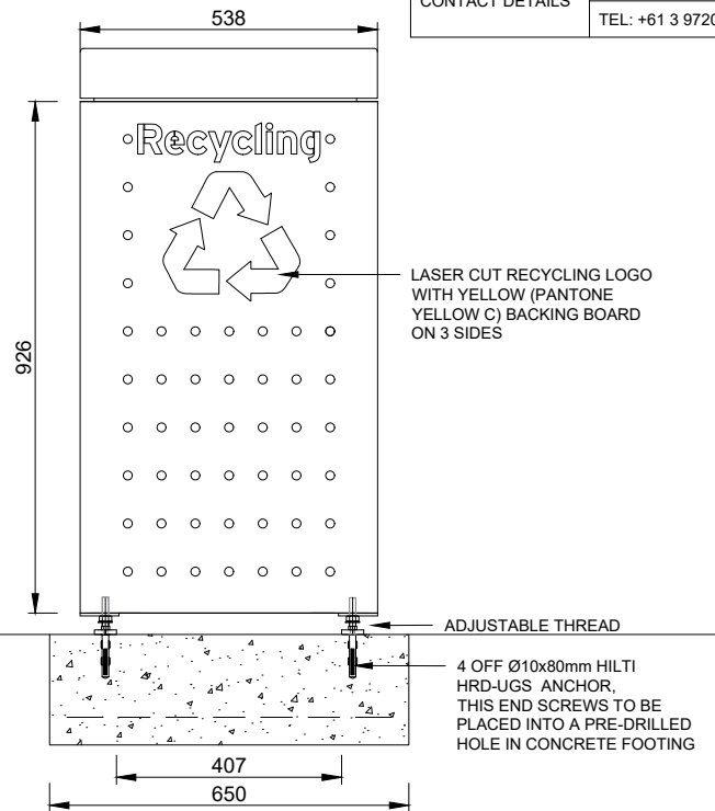
C ELEVATION
