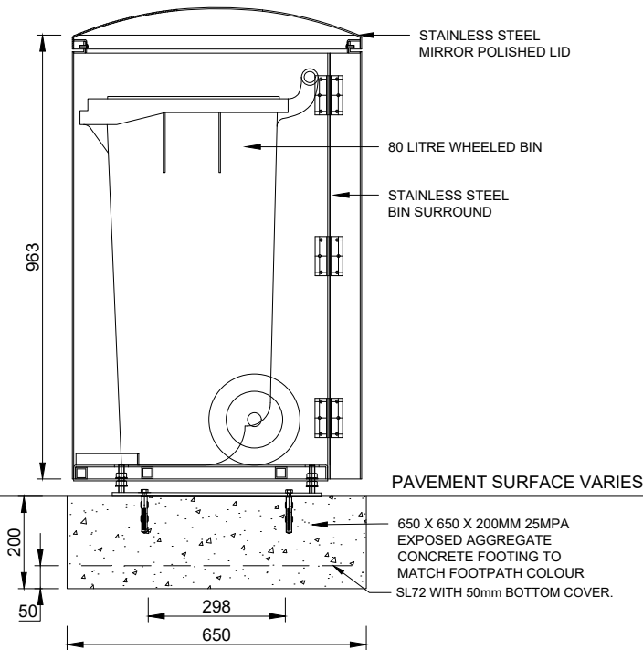
B SECTION
