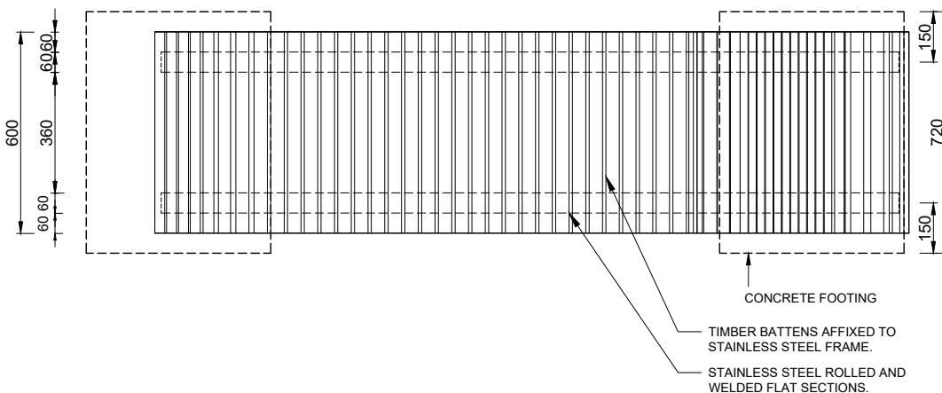
(B) PLAN
