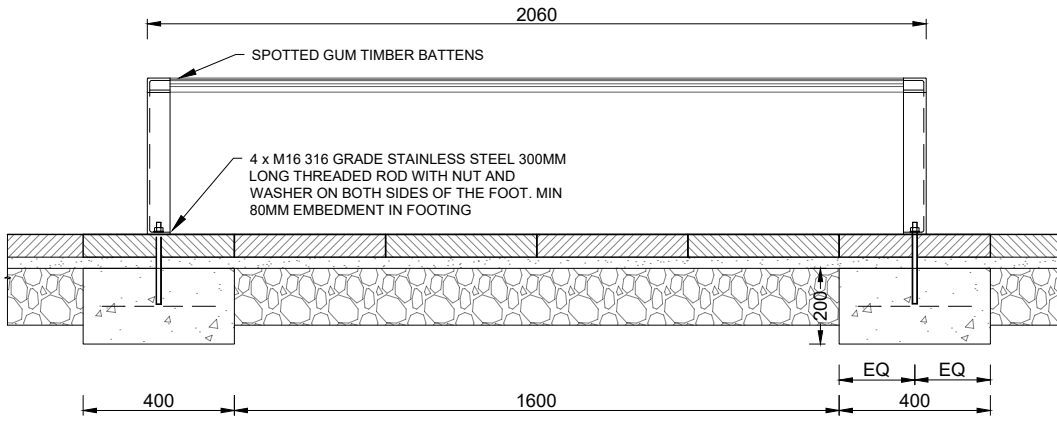
B FRONT ELEVATION
