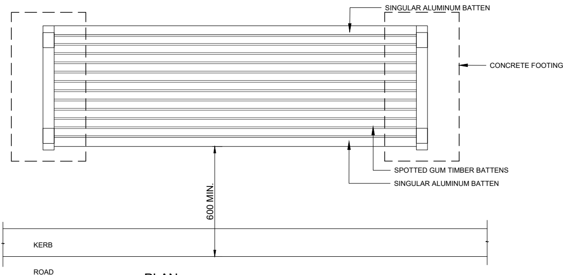
C PLAN
