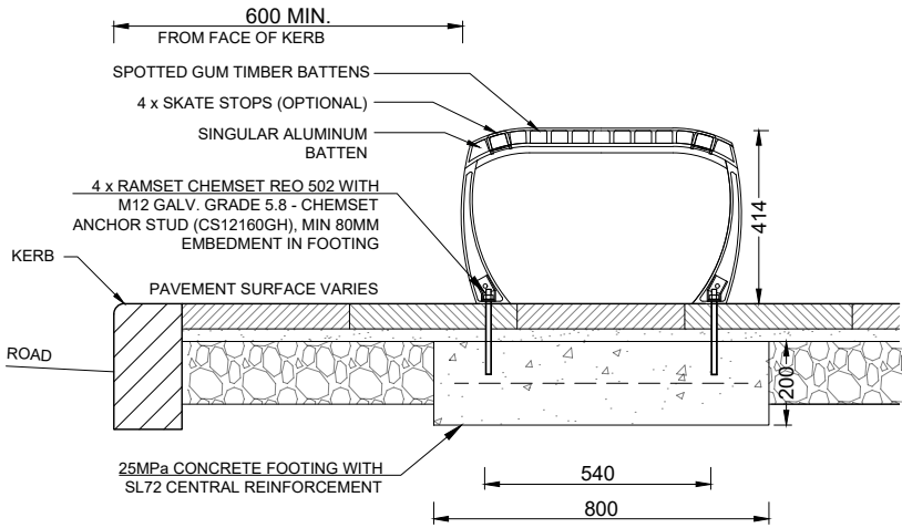
A SECTION
