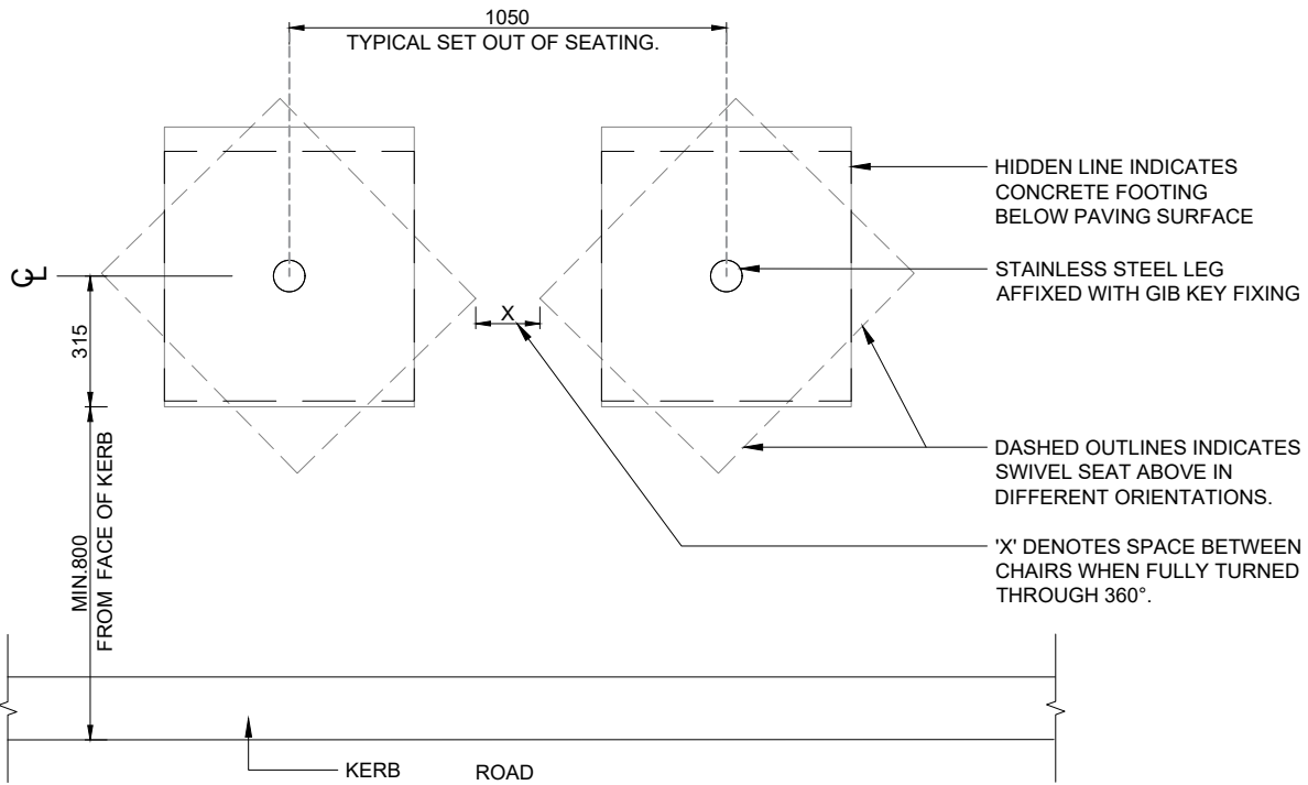
A INDICATIVE LAYOUT PLAN REFER TO PROJECT LAYOUT PLANS FOR SPECIFIC PLACEMENT OF FURNITURE.
