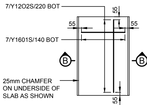
PLAN OF CORBEL SLAB
