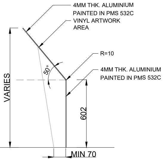
SIDE ELEVATION
