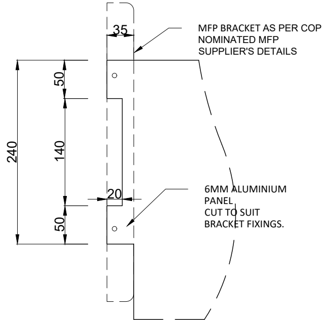
TYPICAL DETAIL
