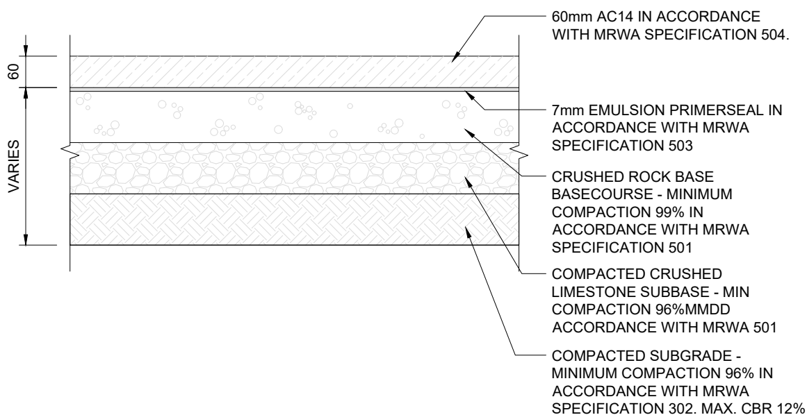
FLEXIBLE PAVEMENT WITH ASPHALT
