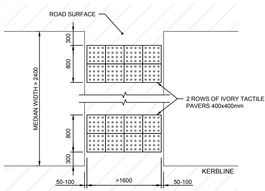
WIDE MEDIAN GAP DETAIL. WIDTH > 2400
