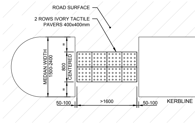
NARROW MEDIAN GAP DETAIL. WIDTH 1500-2400
