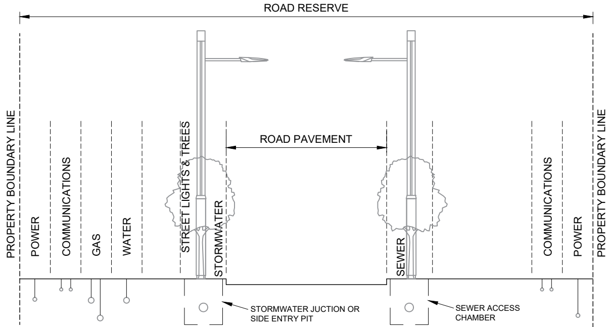
ROAD RESERVE ALLOCATION FOR UTILITY PROVIDERS IN NARROW ROADS
