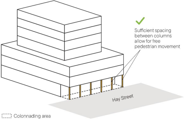
Figure 5. Sufficient spacing between columns within the colonnading area is supported
